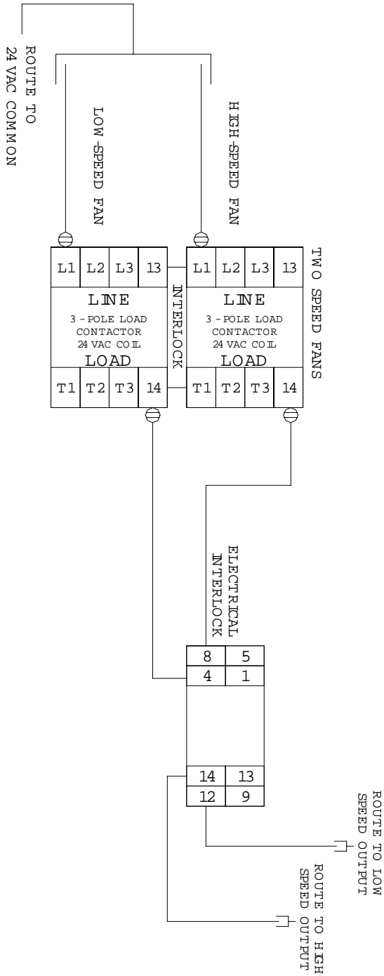
TYPICAL CONNECTION FOR 2 SPEED LOAD CONTACTOR USED FOR 2 SPEED FANS
